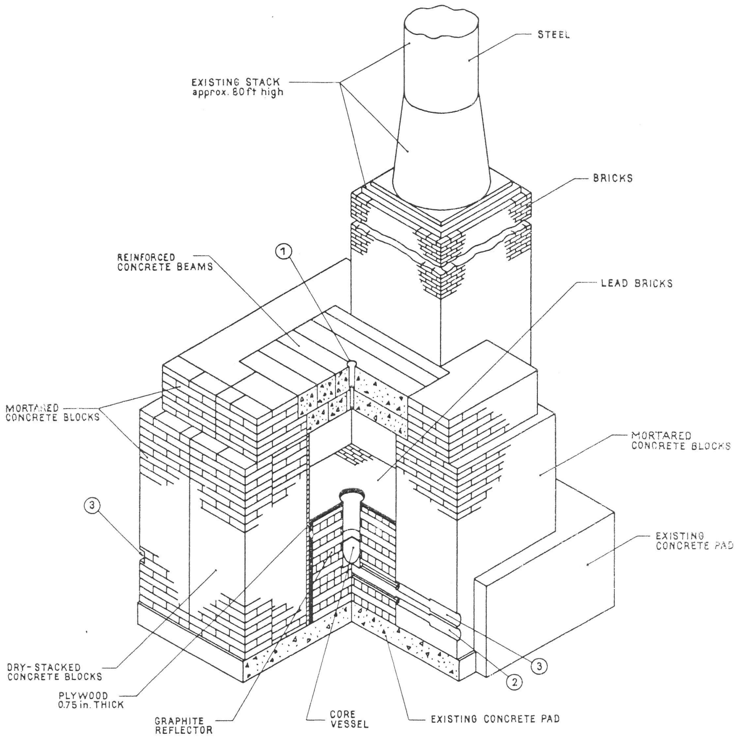
CUTAWAY VIEW NCSCR-4
