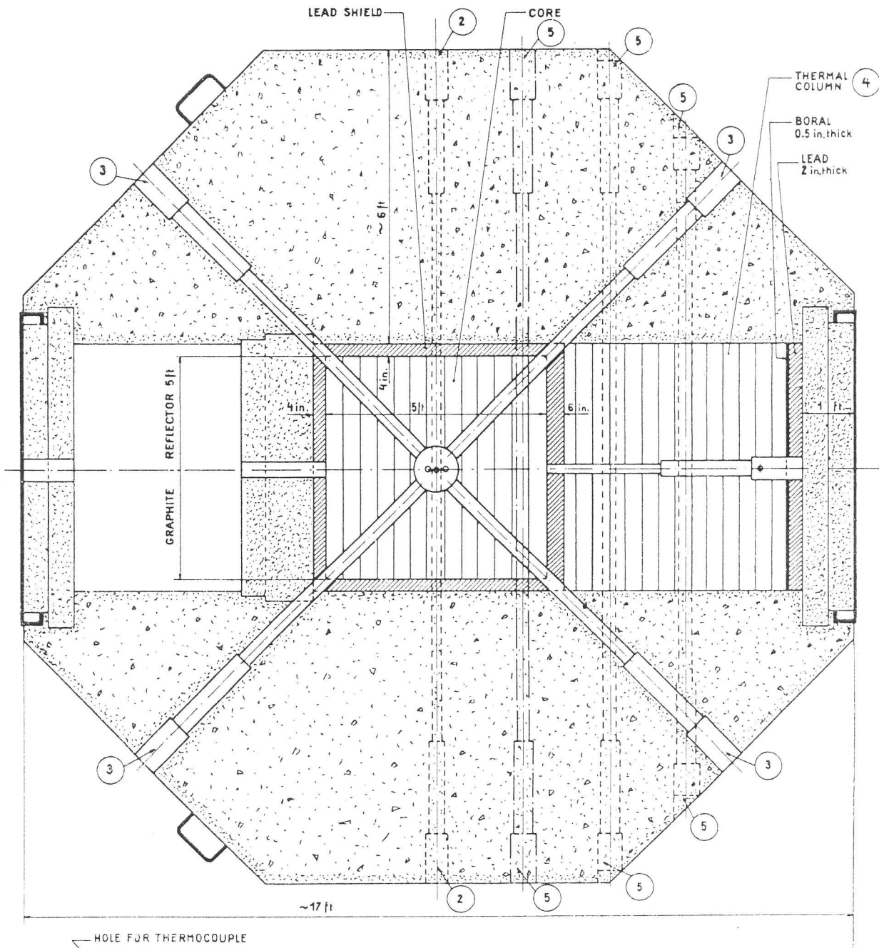
HORIZONTAL SECTION REACTOR NCSCR-2
