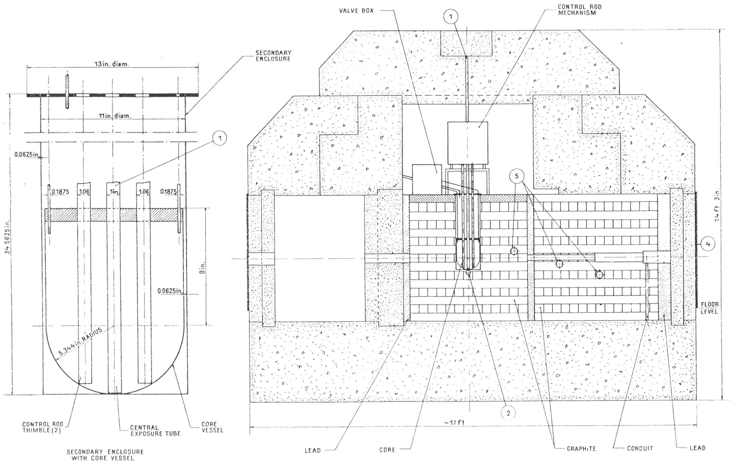
VERTICAL SECTION REACTOR NCSCR-2
